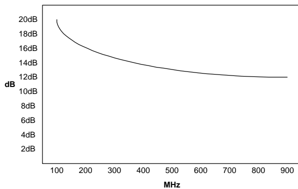
Before 3110 Tilt Compensator
