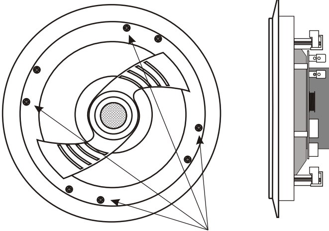
Mounting screws (4)
