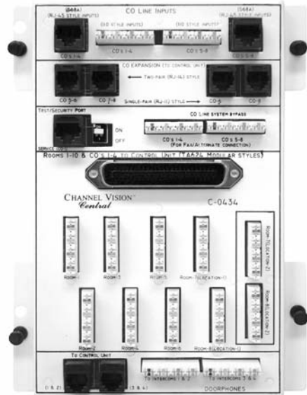
C-0434 KSU Interface Module
